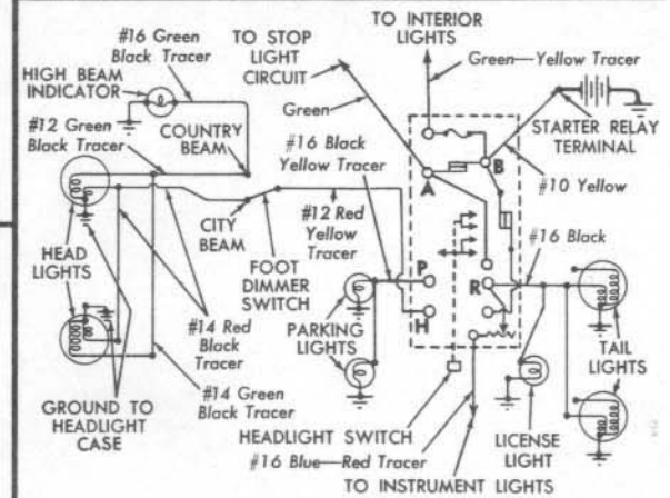
Head Light Circuit Diagram
