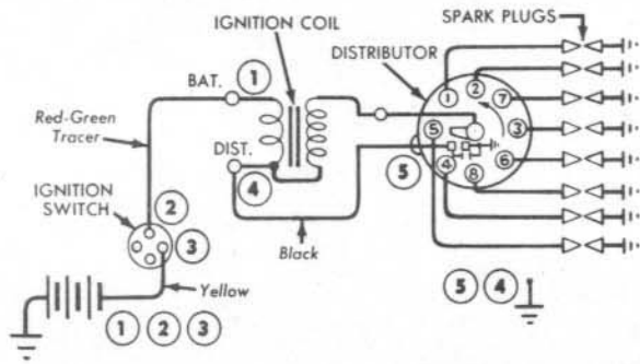
Fig. 2—Ignition Wiring—8-Cylinder Engine
