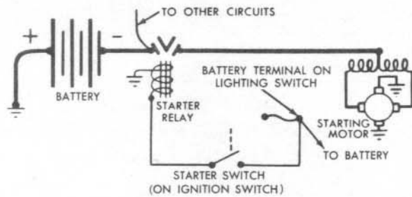
Starting Circuit—Schematic
