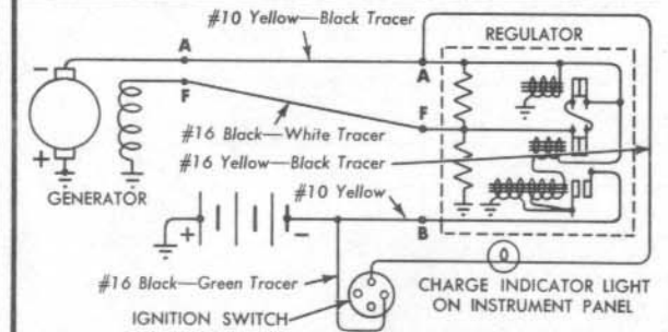
Generator Charge Indicator Light Circuit
