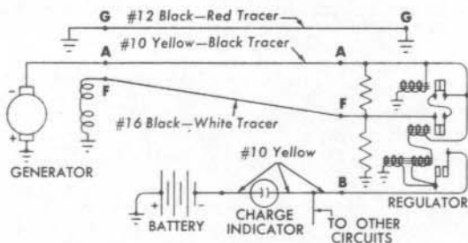
Generating System Circuit—Schematic
