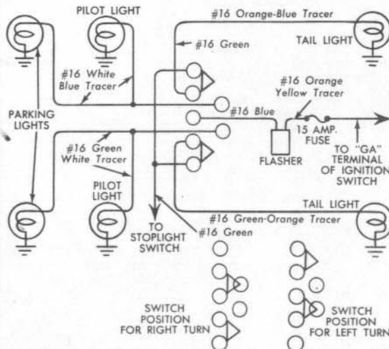
Turn Signal Schematic Diagram
