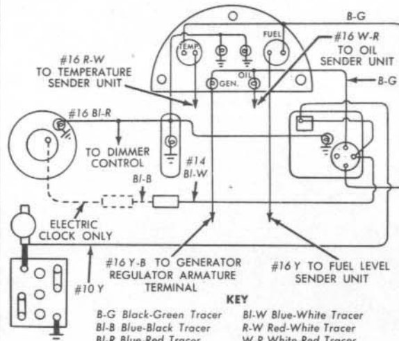
Instrument Cluster Circuit
