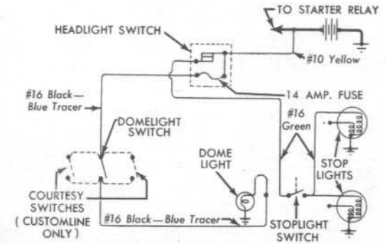
Domelight and Stoplight Diagram
