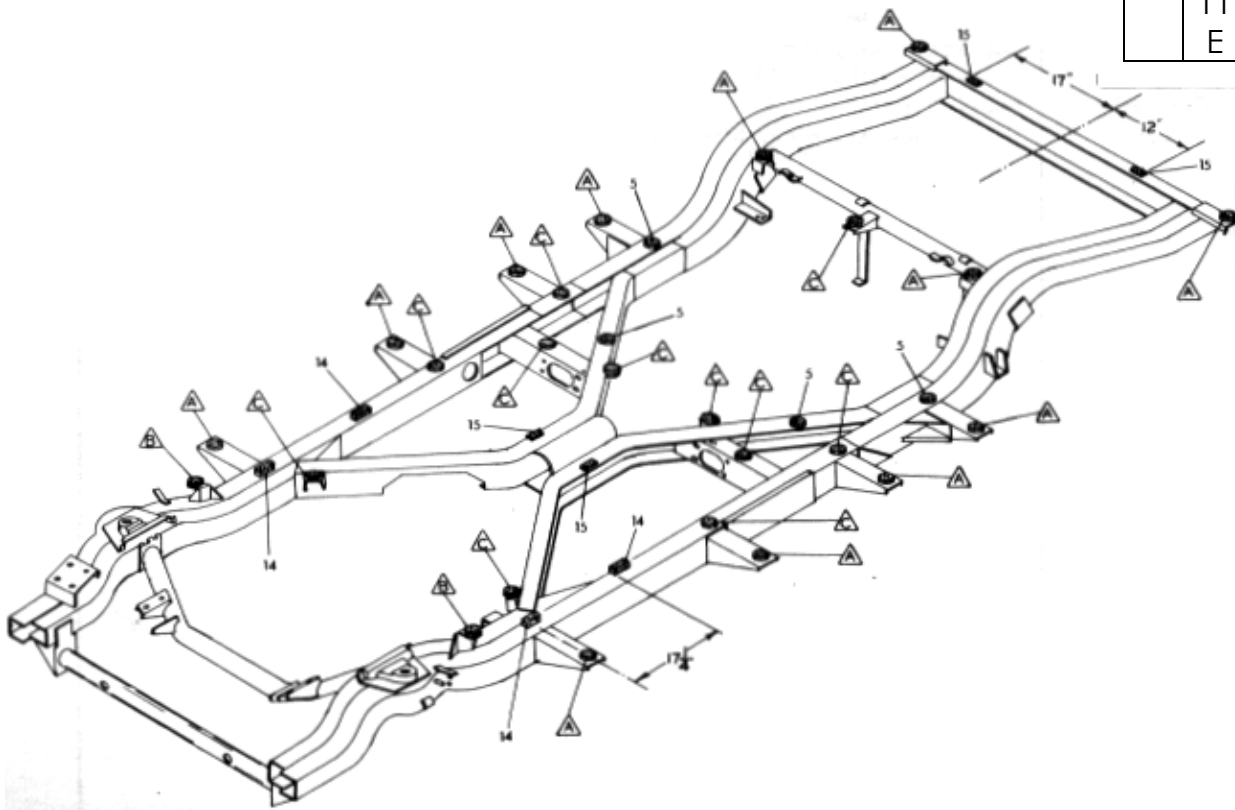
Figure 25-7 Mounting .Body 129" WB
