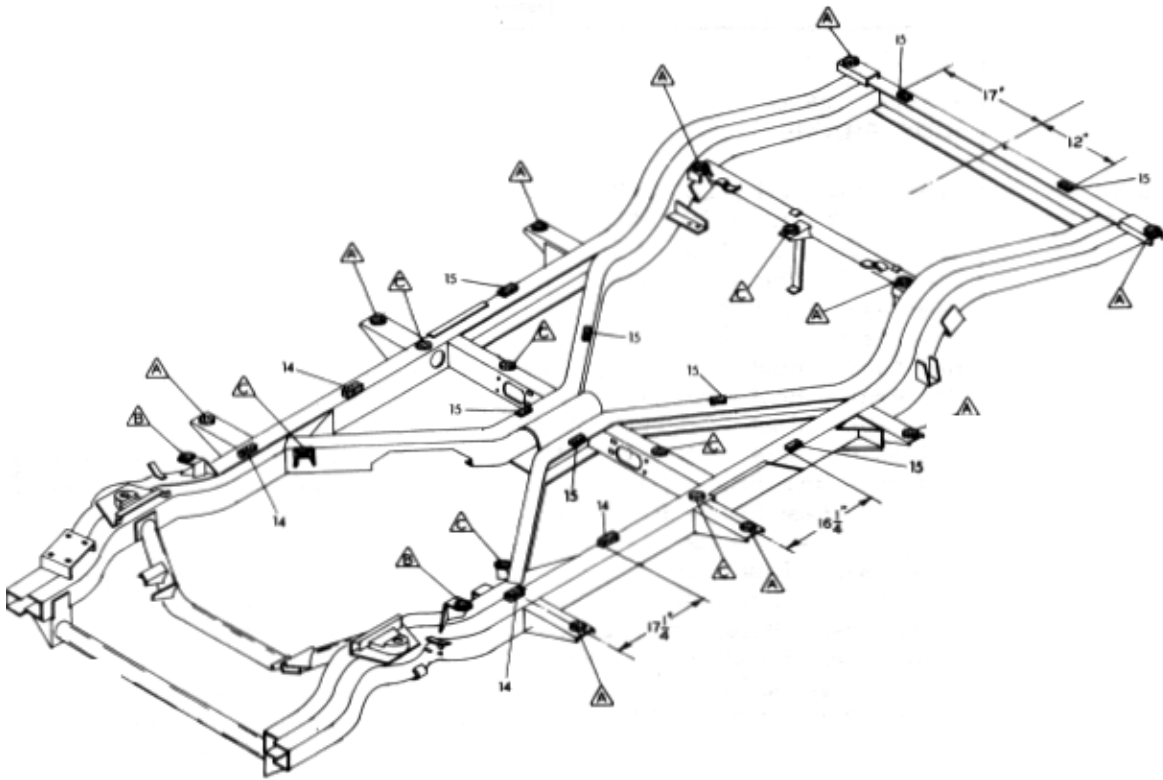
Figure 25-6 Mounting .Body 120" WB
