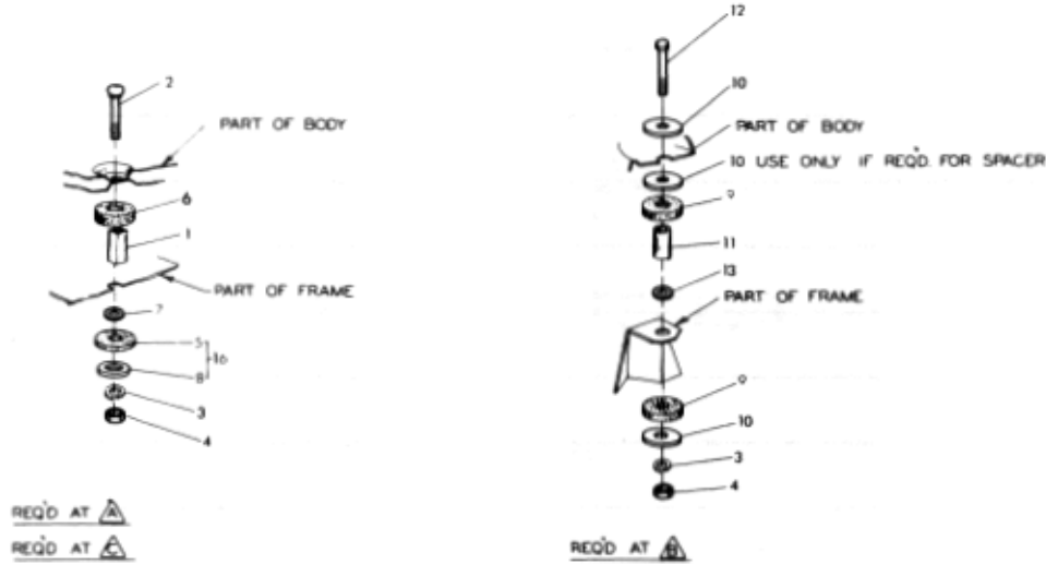
Figure 25-8 Mounting Body
