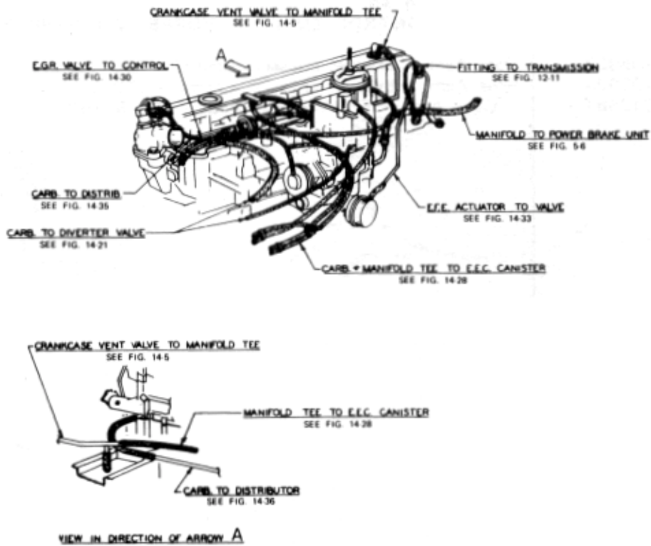
Figure 14-38 Vacuum Lines - General Routing. 6 Cylinder - California
