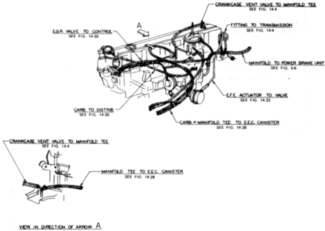
Figure 14-37 Vacuum Lines - General Routing. 6 Cylinder - Federal
