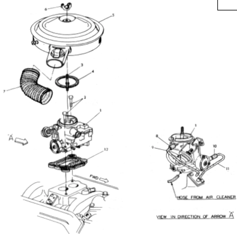
Figure 14-2 Carburetor & Air Cleaner, 305 8 Cylinder Checker Motors Corp.
