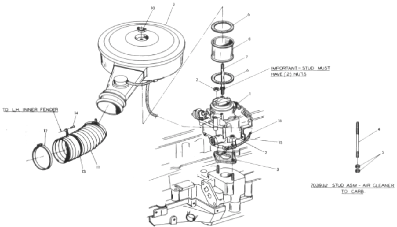
Figure 14-1 Carburetor & Air Cleaner, 6 Cylinder
