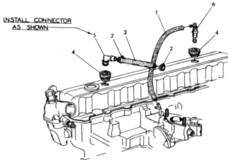
Figure 14-4 Crankcase Ventilation, 6 Cylinder .Federal
