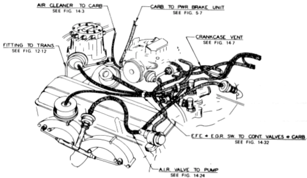
Figure 14-40 Vacuum Lines General Routing. 8 Cylinder -350
