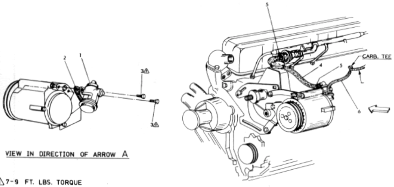
Figure 14-2 1 A.I.R. Hoses. 6 Cylinder
