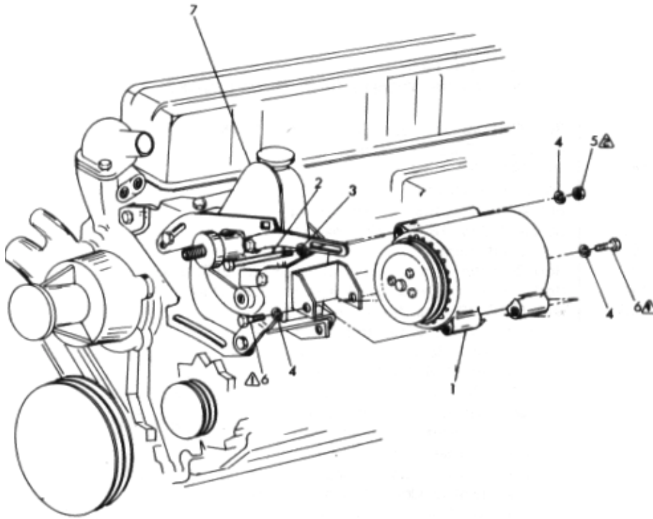
Figure 14-19 A.I.R. Pump Mounting. 6 Cylinder
