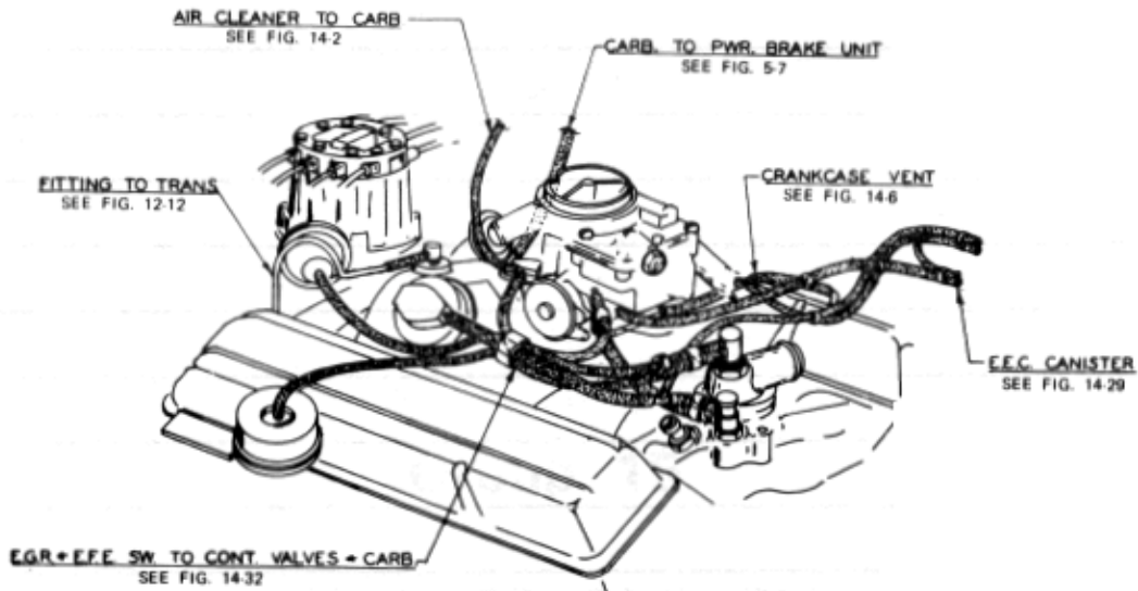
Figure 14-39 Vacuum Lines General Routing. 8 Cylinder -305
