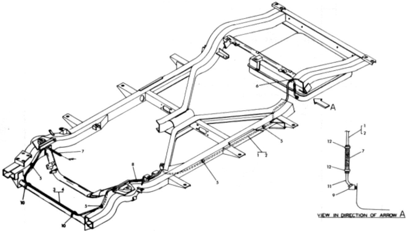
Figure 14-15 Fuel Lines & Fittings, 6 & 8 Cylinder
