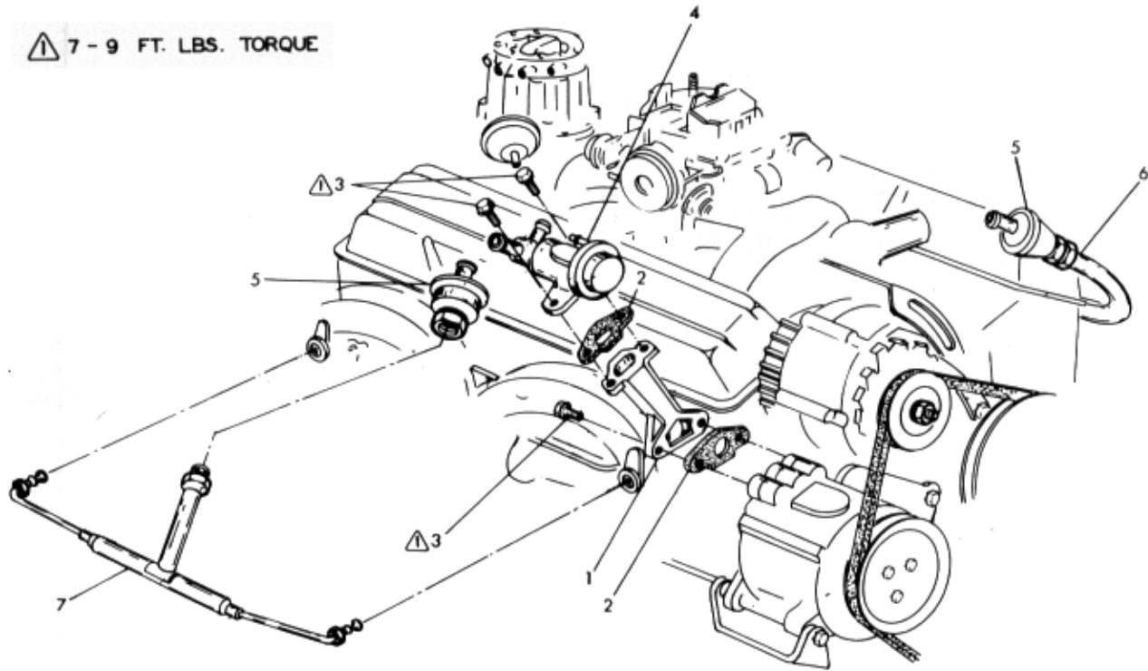
Figure 14-23 A.I.R. Pipe. 350 .8 Cylinder
