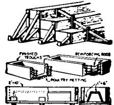
FIG. 4. How to make forms for steps and for water troughs.
