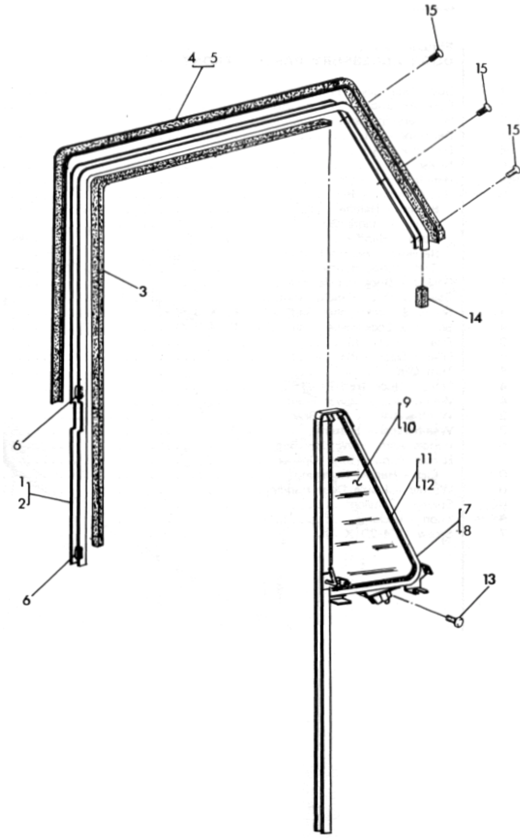
Figure 27-3 Front Door Window Assembly, Frame and Vent Window
