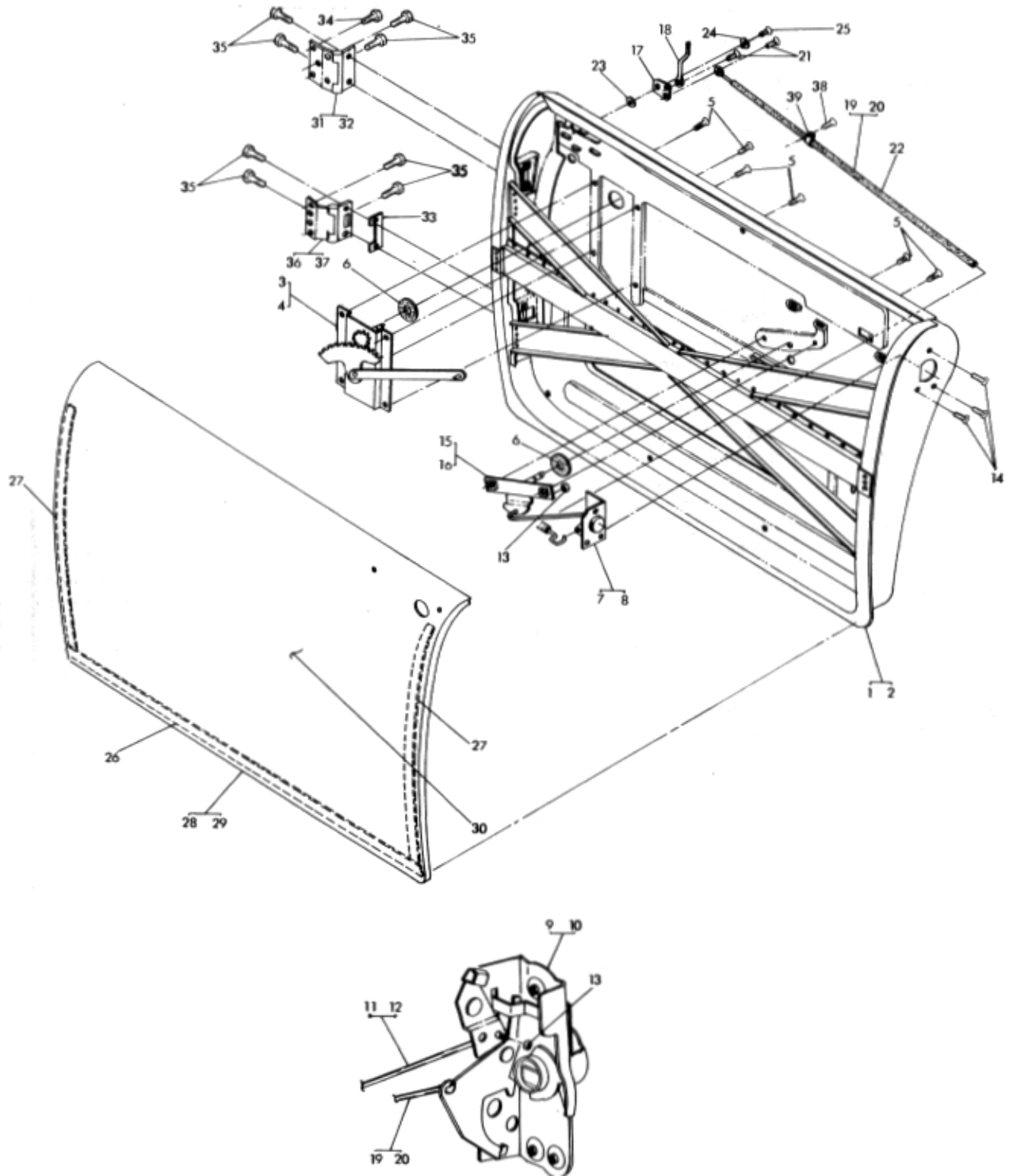
Figure 27-5 Door Assembly .Rear
