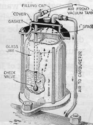
Fig. 5. This simple device for feeding water vapor into the cylinders to cut down carbon deposit works automatically
