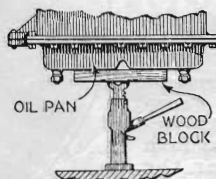
Fig. 8—How a jack can be used to aid in removing or replacing the oil pan of your auto engine
